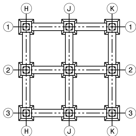
MEMBER AT 1-1, 2-2, 3-3
