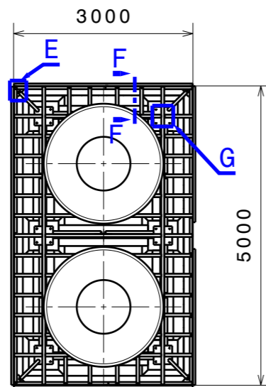
PLAN VIEW AT TANK
