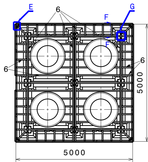
PLAN VIEW AT TANK PLATFORM LEVEL
