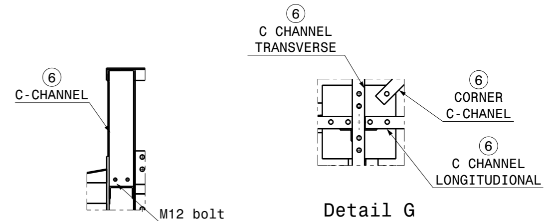
SECTION F-F
