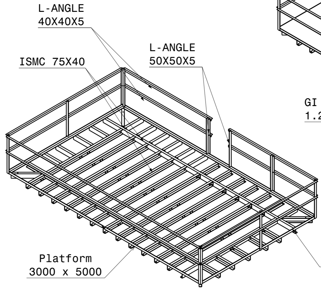
Isometric view of platform
