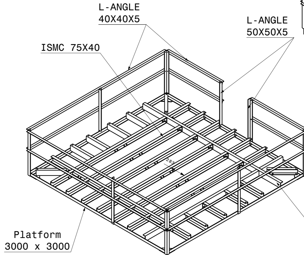
Isometric view of platform
