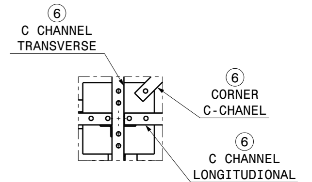
Detail G
