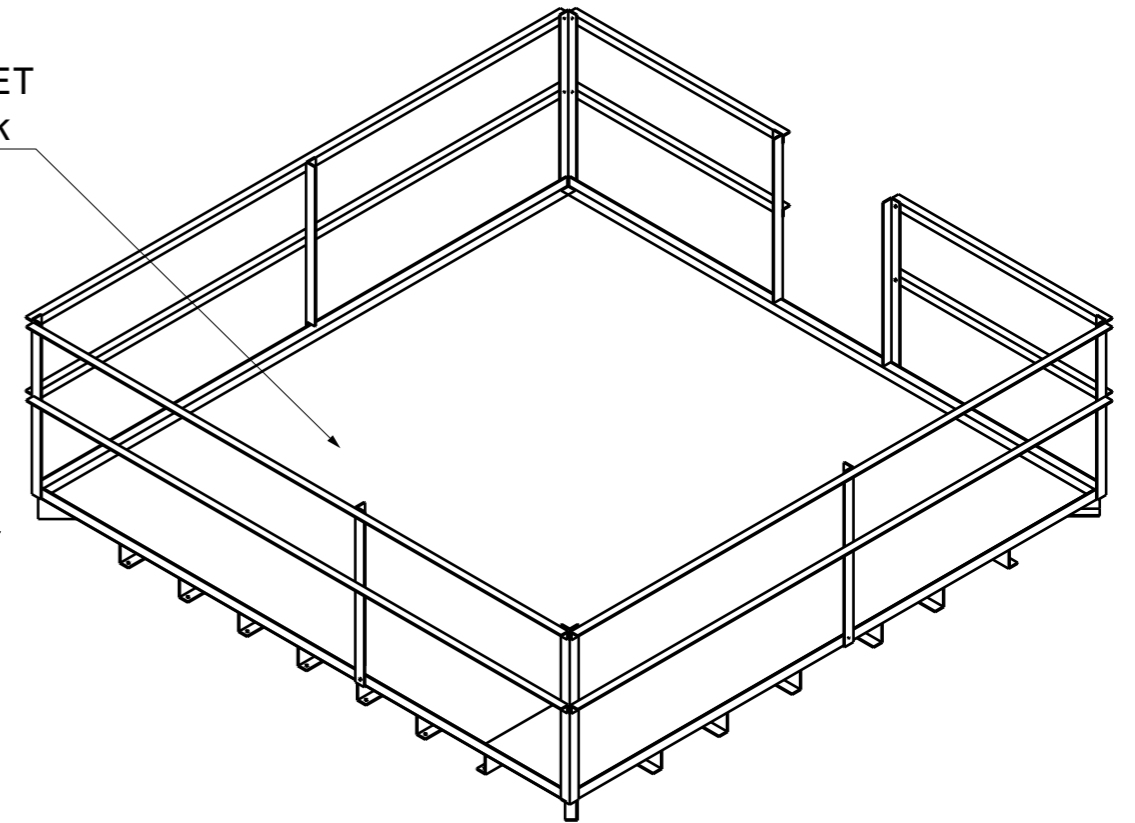
Isometric view of platform with 1.2thk GI sheet
