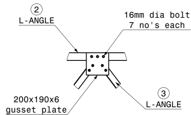
Detail C
