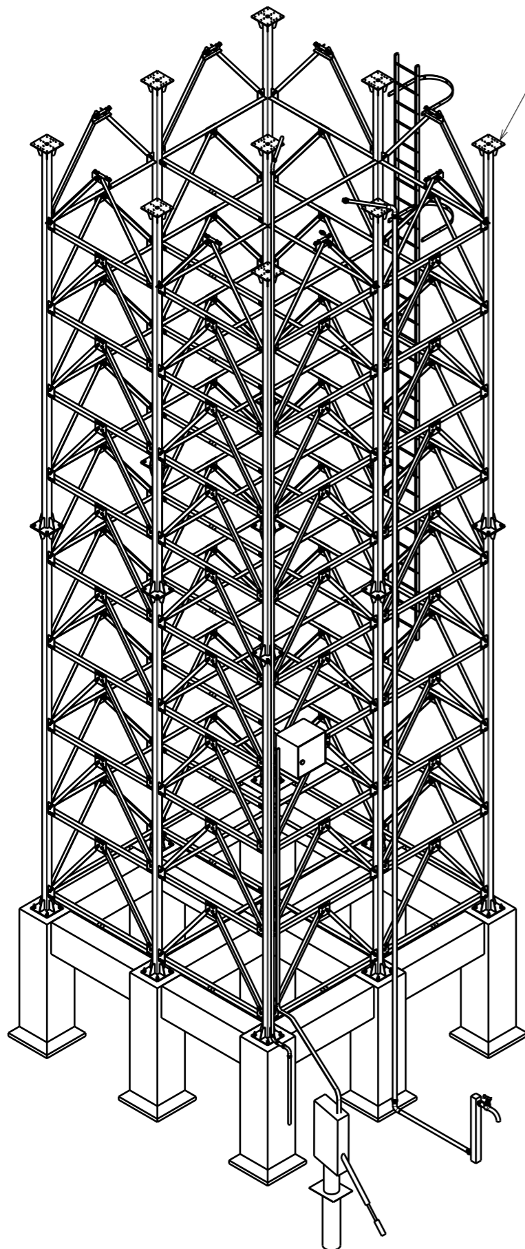
Isometric view OF STRUCTRE
