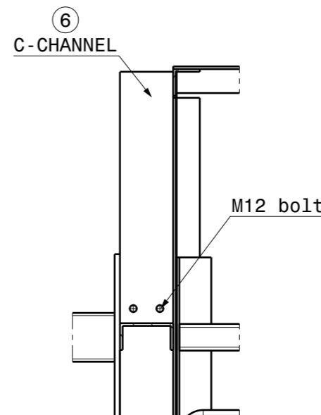
Section F-F
